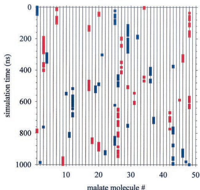
FIGURE 3 History of malate molecules during the 1- \mu s equilibration period of a 10-mM (\text{Na})_2\text{malate} solution. Each vertical line plots the history of a different malate. Red and blue squares indicate times at which the malate is occupying the first and second CS active sites, respectively. Note that the size of the square symbols exaggerates the apparent length of time in which malates occupy the active sites.
